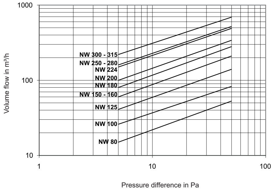
Diagramm1: Pressure loss of the weather louvre in the exhaust air
