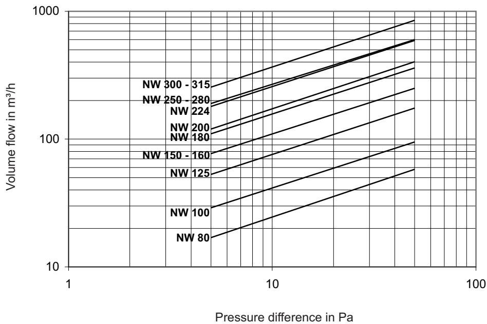
Diagramm1: Pressure loss of the weather louvre in the supply air
